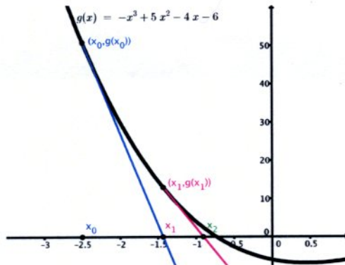
Figure 1: Newton's method
