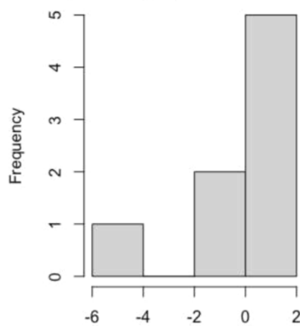
Histogram of p8_11.model1$residuals
