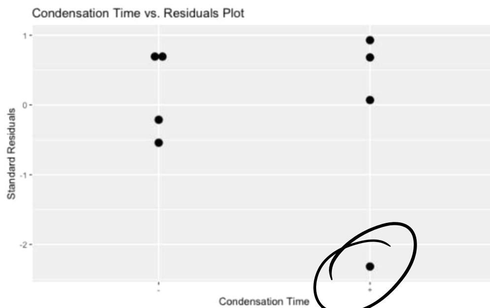
Figure 13: Residuals vs. Factor B
