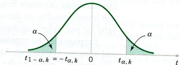
Figure 8-5 Percentage points of the t distribution.
