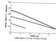
Figure 4. A typical output from Eq. (1). Shows are initial and launch angles for prescribed range values.
