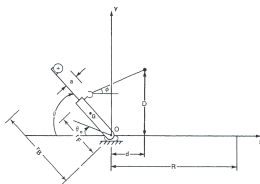
Figure 2. Schematic of the catapult with dimensions.
