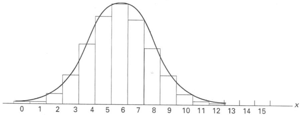
Figure 6.22 Normal approximation of b(x; 15, 0.4) .
